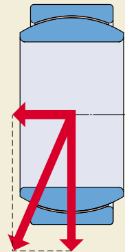
Combined (radial and axial) acting load
